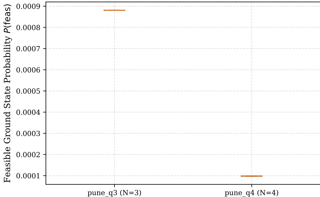
QAOA Ground State Sampling Probability (Corrected Closed-Tour QUBO)
